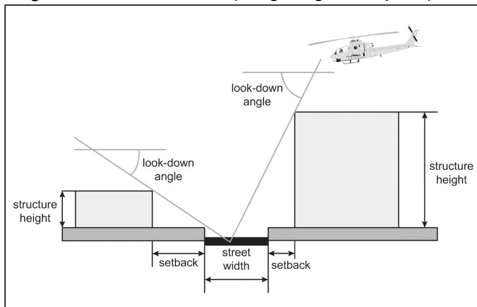
Figure 19. Look-Down Angle
